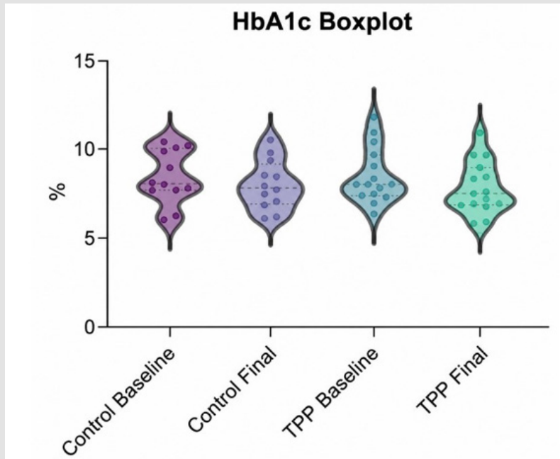
Figure 4: Boxplot and violin plot showing the distribution of HbA1c across study groups at both baseline and final visits.
