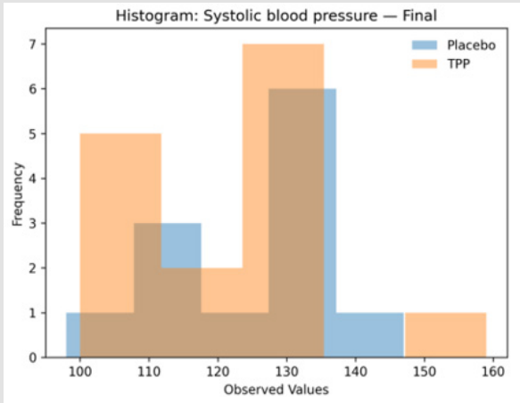
Supplementary Figure S2d: Histograms — Systolic blood pressure, Final.
