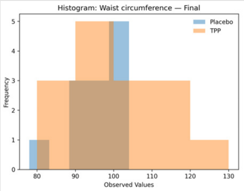
Supplementary Figure S2f: Histograms — Waist circumferesnce, Final.
