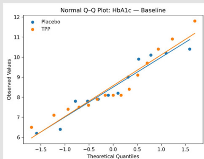
Supplementary Figure S1a: Normal Q-Q plots — HbA1c, Baseline.
