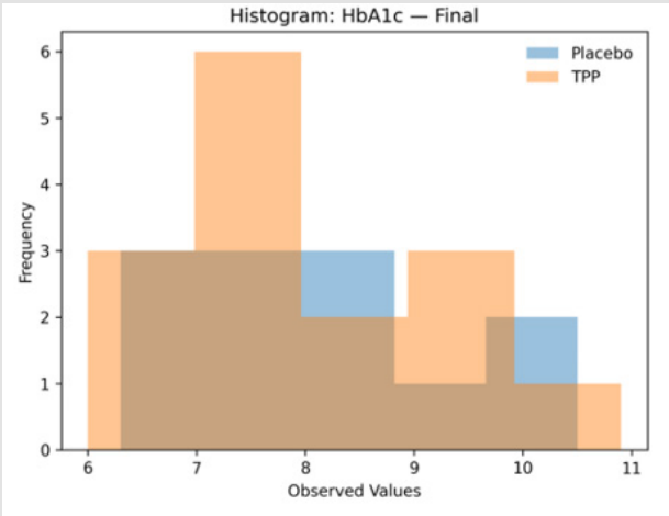
Supplementary Figure S2b: Histograms — HbA1c, Final.
