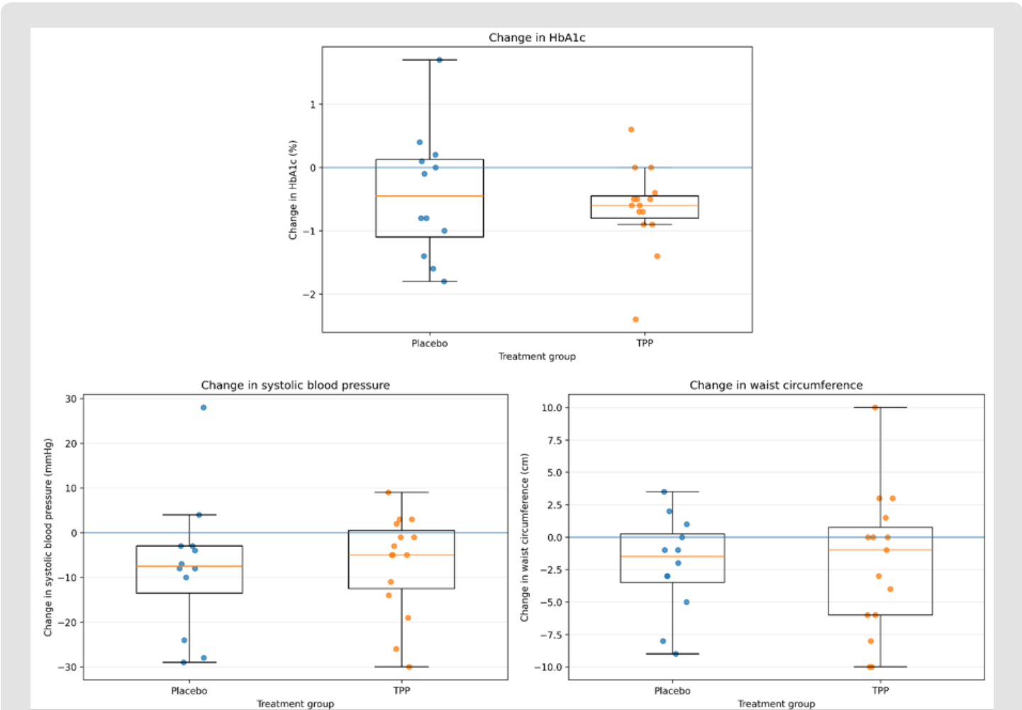
Figure 2: Changes in HbA1c, systolic blood pressure, and waist circumference from baseline to final assessment by treatment group.
