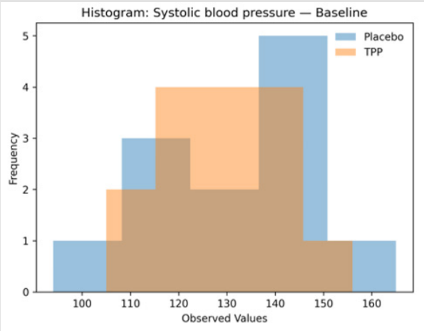
Supplementary Figure S2c: Histograms — Systolic blood pressure, Baseline.
