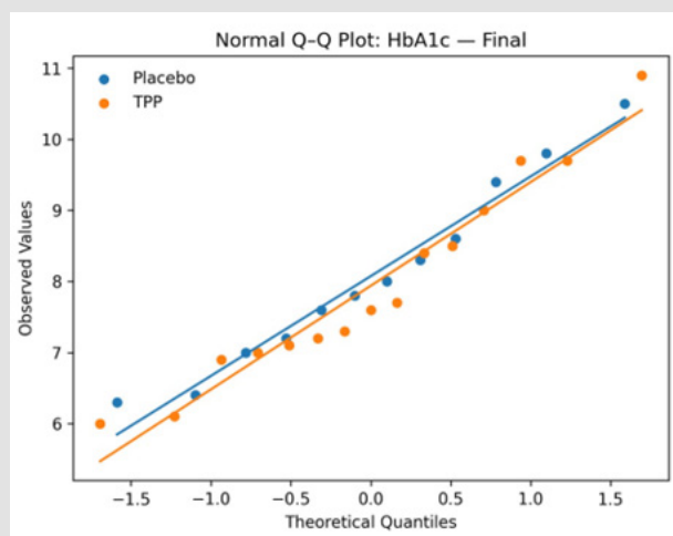
Supplementary Figure S1b: Normal Q-Q plots — HbA1c, Final.
