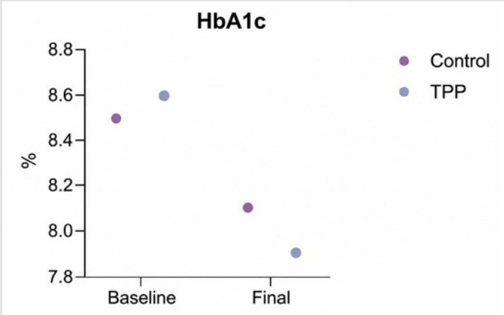
Figure 3: Trend in HbA1c evolution between the control and experimental groups.
