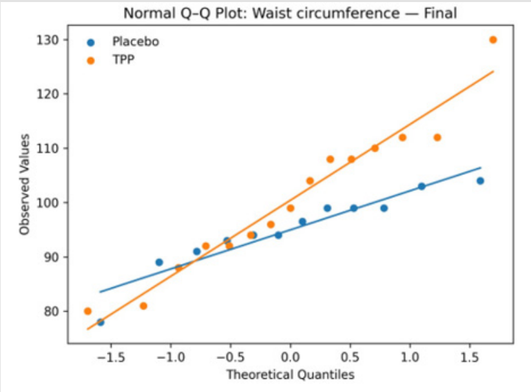
Supplementary Figure S1f: Normal Q-Q plots — Waist circumference, Final.
