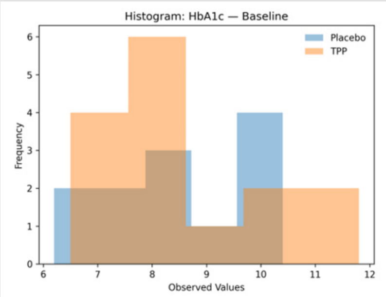
Supplementary Figure S2a: Histograms — HbA1c, Baseline.
