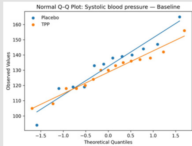
Supplementary Figure S1c: Normal Q-Q plots — Systolic blood pressure, Baseline.
