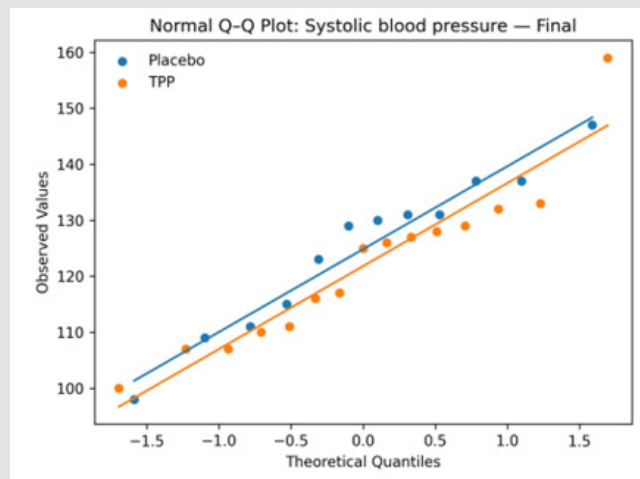
Supplementary Figure S1d: Normal Q-Q plots — Systolic blood pressure, Final.
