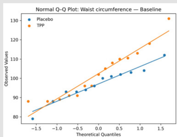
Supplementary Figure S1e: Normal Q-Q plots — Waist circumference, Baseline.
