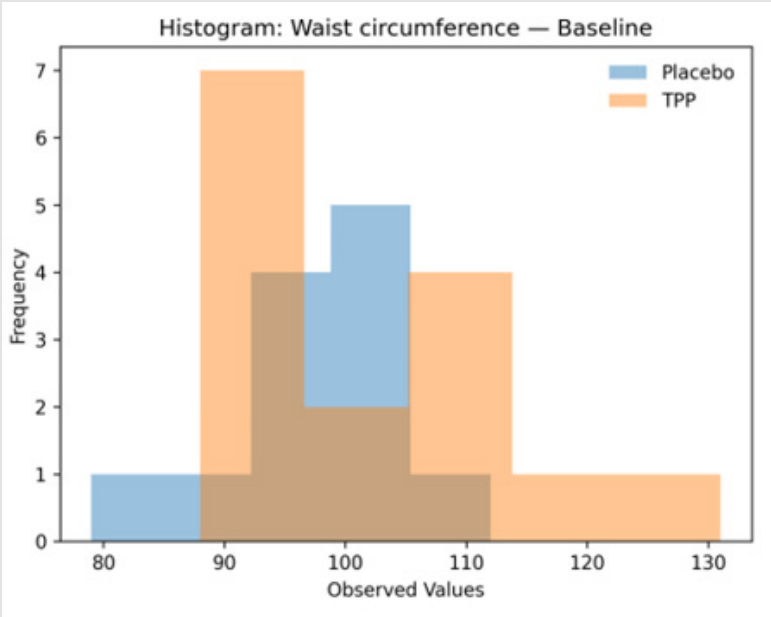
Supplementary Figure S2e: Histograms — Waist circumference, Baseline.
